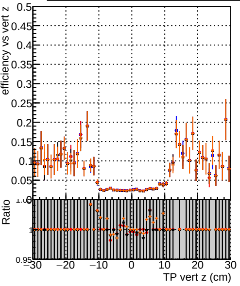
Efficiency vs vertpos DOM_test_CKF-FitDefault DOM_test_mkFitFit DOM_test_mkFitFit_noOL DOM_test_mkFitNOFit_retest
