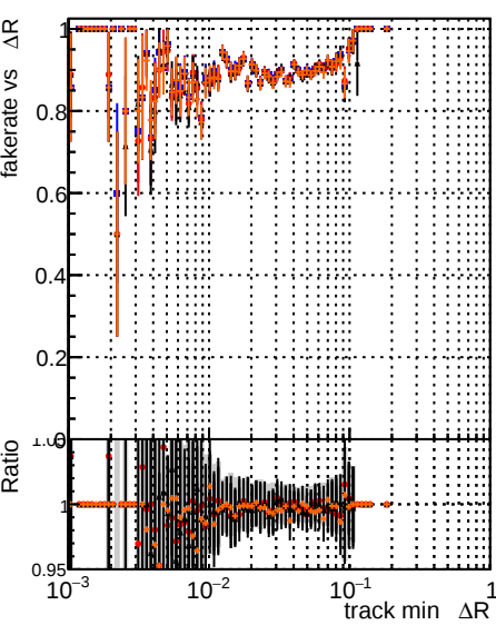
Fake rate vs \Delta R(\text{track, jet}) Legend: DOM test CKFit Default DOM test CKFit noOL DOM test mktFit DOM test mktFit retest
