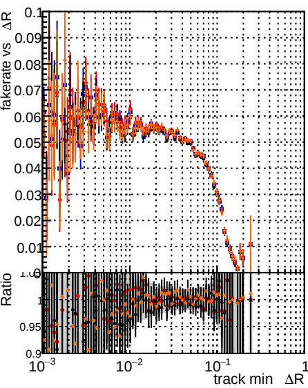
Fake rate vs \Delta R(\text{track, jet}) Legend: DOM jet CKKF fit Default DOM jet mktfit noOL DOM jet mktfit retest
