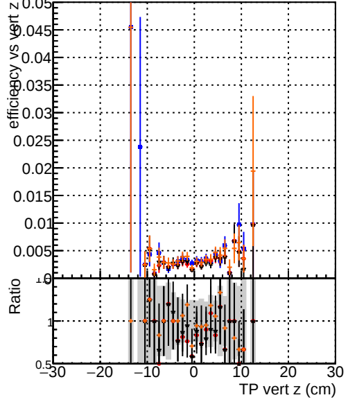
Efficiency vs. TP vert z (cm) — DOM_test_CKFfitDefault — DOM_test_mkFitFit — DOM_test_mkFitFit_noOL — DOM_test_mkFitNOFit_retest
