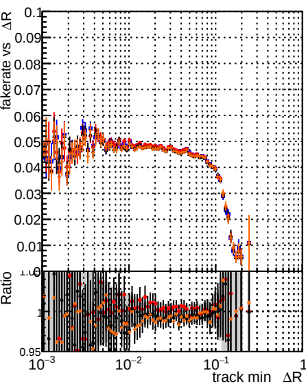
Fake rate vs \Delta R(\text{track}, \text{jet}) Legend: DOM test CKFit Default DOM test mktFit noOL DOM test mktFit retest
