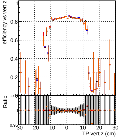
Efficiency vs. sim PV z DOM_test_CKFfitDefault DOM_test_mkFitFit DOM_test_mkFitFit_noOL DOM_test_mkFitNOFit_retest
