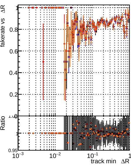
Fake rate vs \Delta R(\text{track, jet}) Legend: DOM test CKFit Default DOM test mktFit noOL DOM test mktFit NOFit retest
