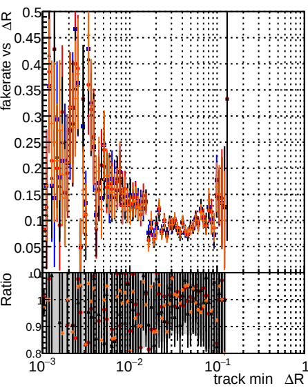
Fake rate vs \Delta R(\text{track, jet}) Legend: DOM jet CKFit Default DOM jet CKFit noOL DOM jet mktFit DOM jet mktFit retest
