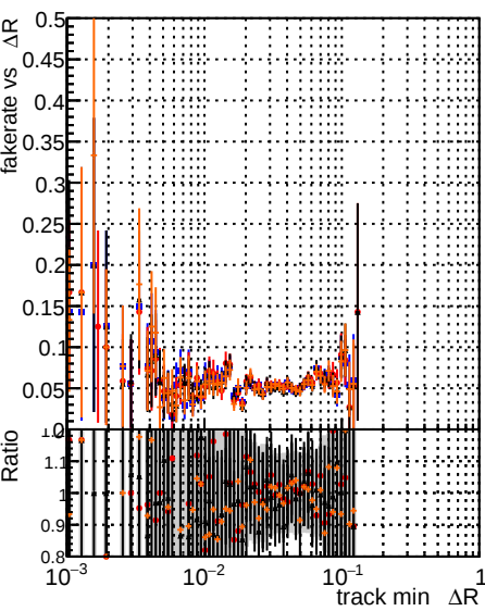
Fake rate vs \Delta R(\text{track, jet}) Legend: DOM jet CKF Fit Default DOM jet CKF Fit noOL DOM jet CKF Fit retest
