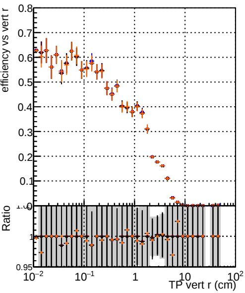
Efficiency vs TP vert r (cm) DOM_test_CKFitDefault DOM_test_mkFitFit DOM_test_mkFitFit_retest DOM_test_mkFitNOFit_retest
