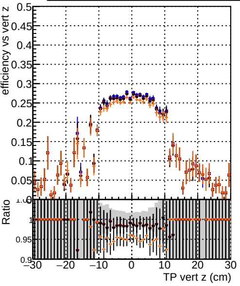
Efficiency vs vertpos Legend: DOM_test_CKFitDefault DOM_test_mkFitFit DOM_test_mkFitFit_retest DOM_test_mkFitNOFit_retest
