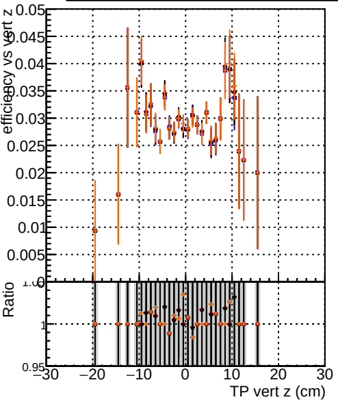
Efficiency vs vertpos DOM_test_CKF-FitDefault DOM_test_mkFitFit DOM_test_mkFitFit_retest DOM_test_mkFitNOFit_retest
