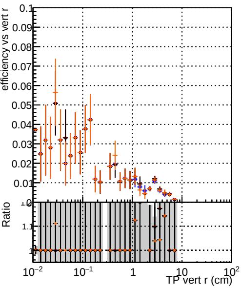
Efficiency vs vertpos Legend: DOM_test_CKFFitDefault DOM_test_mkFitFit DOM_test_mkFitFit_retest DOM_test_mkFitNOFit_retest
