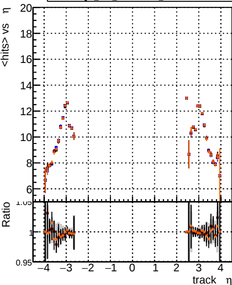
mean hits vs \eta DOM_test_CKFFitDefault DOM_test_mkFitFit DOM_test_mkFitFit_retest DOM_test_mkFitNOFit_retest
