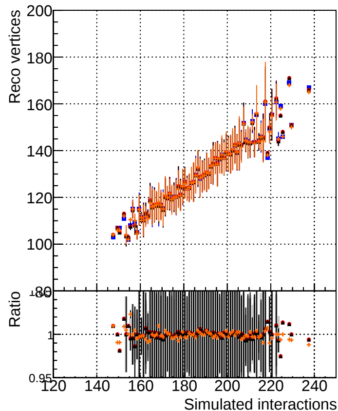
RecoVtx_vs_GenVtx
