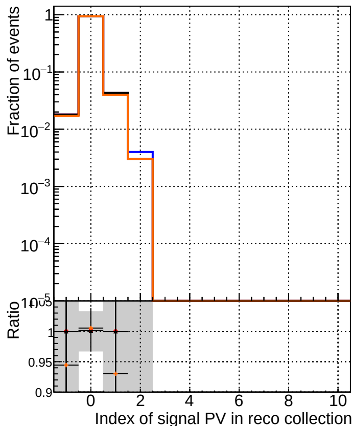
TruePVLocationIndexInRecoVertexCollection
