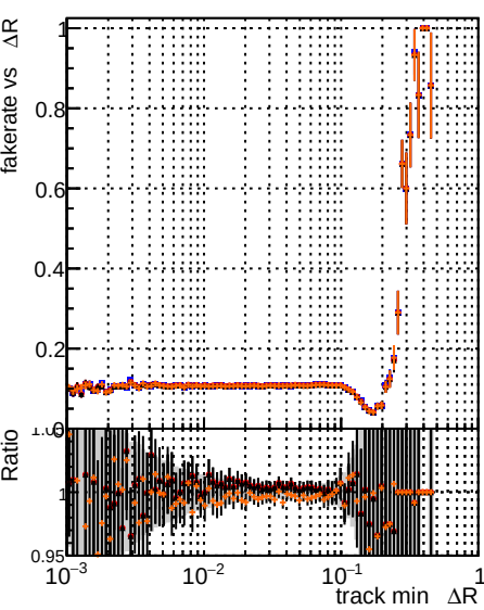
Fake rate vs \Delta R(\text{track, jet}) Legend: DOM, test, CKEF, fit, Default, test, mkt, fit, retest, test, mkt, fit, retest
