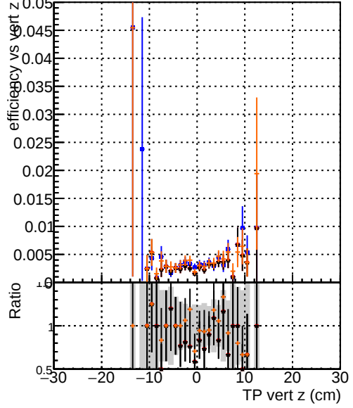
Efficiency vs. sim PV z DOM_test_CKFfitDefault DOM_test_mkFitFit DOM_test_mkFitFit_retest DOM_test_mkFitNOFit_retest
