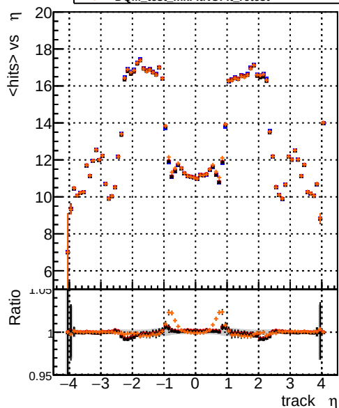
mean hits vs \eta DOM_test_CKFitDefault DOM_test_mkFitFit DOM_test_mkFitFit_retest DOM_test_mkFitNOFit_retest
