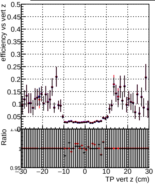
Efficiency vs TP vert z Legend: DQM_test_CKFFitDefault (Blue squares) DQM_test_doubleFit (Red circles) DQM_test_mkFitFit_newOL3 (Black triangles)
