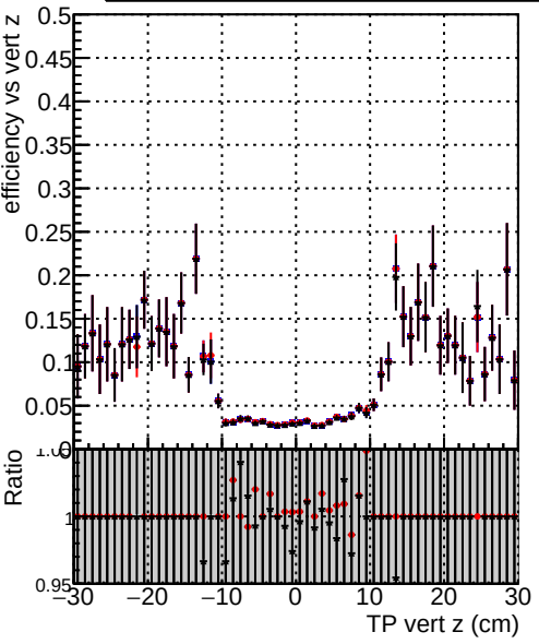
Efficiency vs vertpos Legend: DQM_test_CKFFitDefault DQM_test_doubleFit DQM_test_mkFitFit_newOL3
