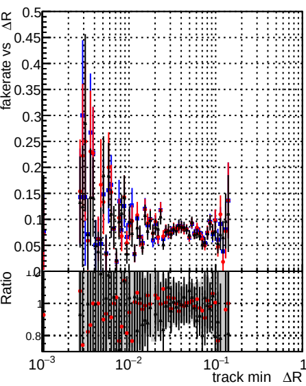
Legend: DQM test CKFitDefault (blue), DQM test doubleFit (red), DQM test mkFitFit_newOL3 (black)
