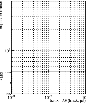
N of associated tracks (recoToSim) looper tracks vs dR(track, jet)
