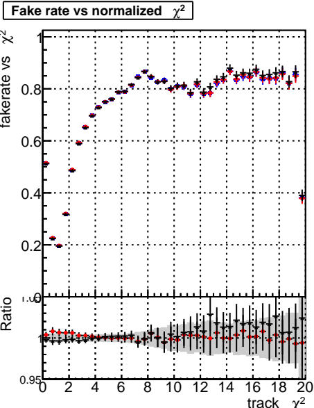
Fake rate vs. \chi^2 █ DCM test CKFFit Default █ DCM test gouFit █ DCM test mkFit newOL3
