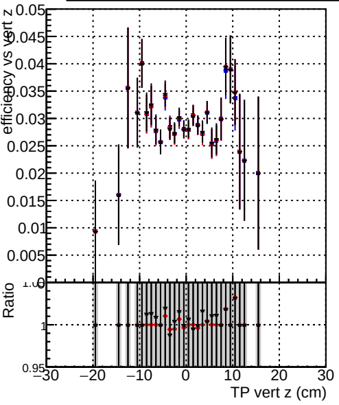
Efficiency vs TP vert z Legend: DQM_test_CKFFitDefault (blue squares) DQM_test_doubleFit (red circles) DQM_test_mkFitFit_newOL2 (black crosses)
