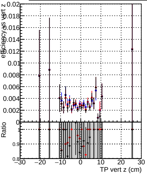
Efficiency vs TP vert z (cm) plot Legend: DQM_test_CKFFitDefault (Blue circles) DQM_test_doubleFit (Red circles) DQM_test_mkFitFit_newOL2 (Black circles)
