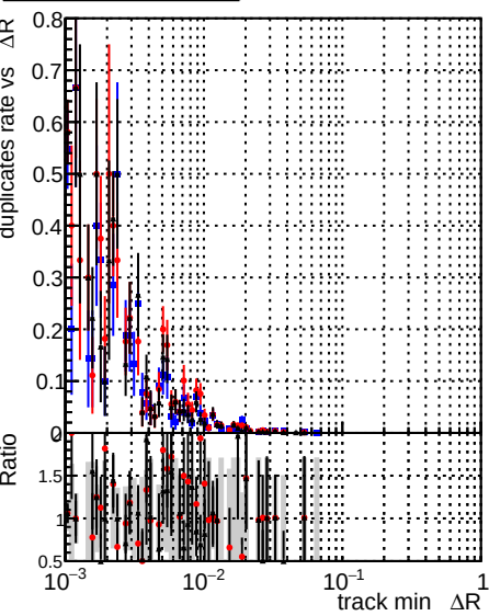
Legend: DQM_test_CKFFitDefault (blue), DQM_test_doubleFit (red), DQM_test_mkFitFit_newOL2 (black)
