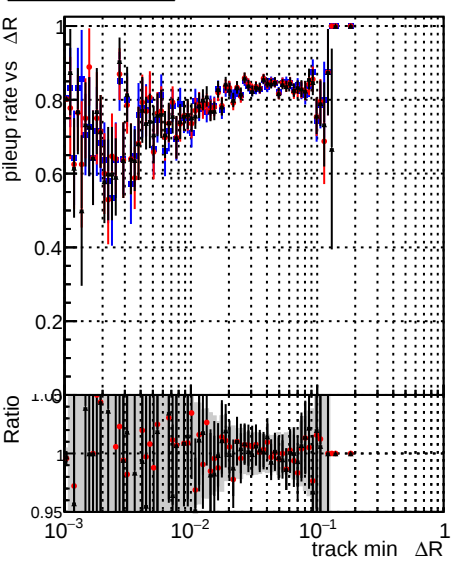
Legend: \bullet DOM_test_CKFFitDefault \bullet DOM_test_doubleFit \bullet DOM_test_mkFitFit_newOL2
