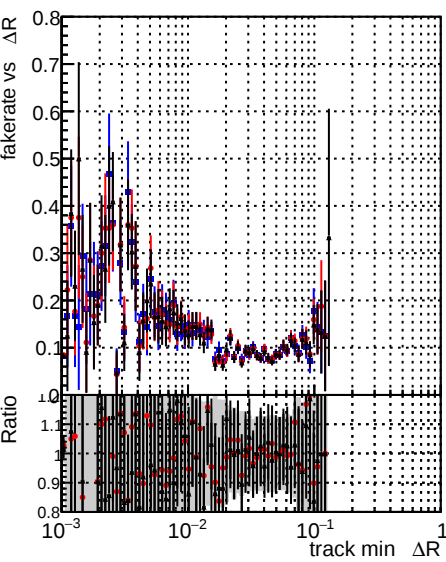
Legend: \bullet DOM_test_CKFFitDefault \bullet DOM_test_doubleFit \bullet DOM_test_mkFitFit_newOL2
