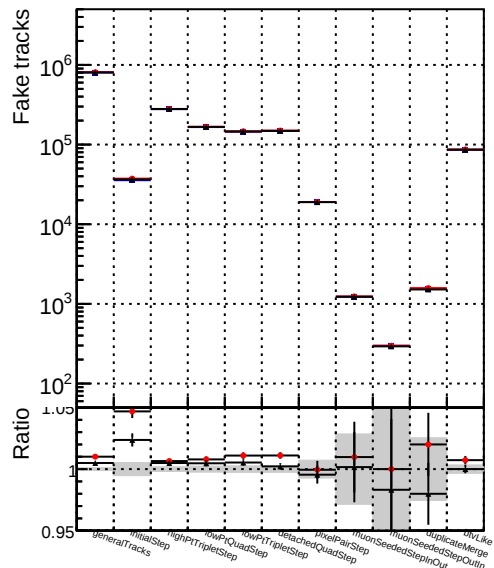
Number of tracks vs collection Legend: DQM_test_CKFFitDefault (blue squares) DQM_test_doubleFit (red circles) DQM_test_mkFitFit_newOL (black circles)
