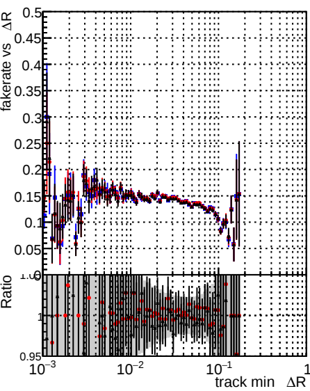
Fake rate vs \Delta R(\text{track, jet}) Legend: \Delta R(\text{track, jet}) (blue line with circles) \Delta R(\text{track, jet}) (red line with circles) \Delta R(\text{track, jet}) (black line with circles)
