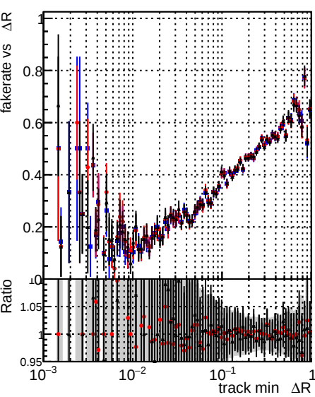
Fake rate vs \Delta R(\text{track, jet}) Legend: DQM_test_CKFFitDefault (blue line with squares) DQM_test_doubleFit (red line with circles) DQM_test_mkFitFit_newOL (black line with triangles)
