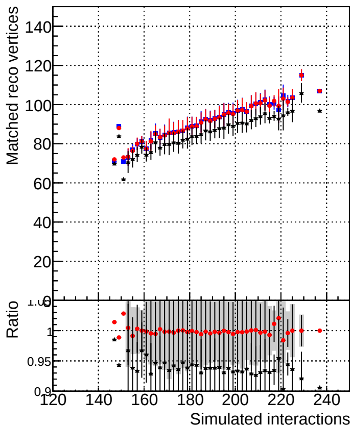
MatchedRecoVtx_vs_GenVtx
