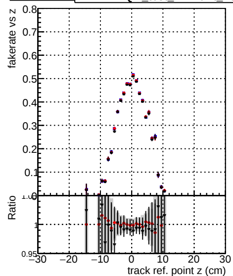
—●— DOM_test_CKFFitDefault —●— DOM_test_doubleFit —●— DOM_test_mkFitFit_noOL
