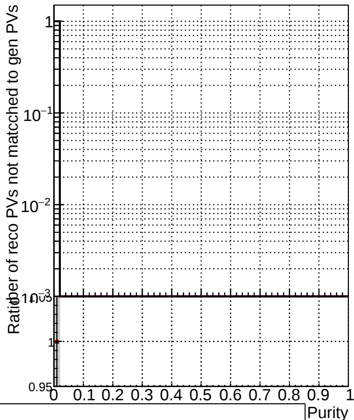
RecoPVAssoc2GenPVNotMatched_Purity
