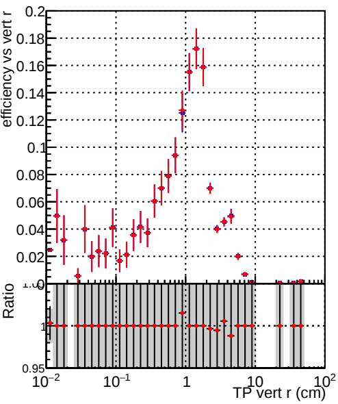
Efficiency vs TP vert r (cm) Legend: DQM_test_CKFFitDefault (blue line with markers) DQM_test_doubleFit (red line with markers)
