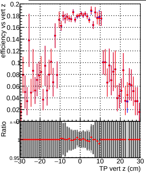
Efficiency vs vert z Legend: DQM_test_CKFFitDefault (blue line with error bars), DQM_test_doubleFit (red line with error bars)
