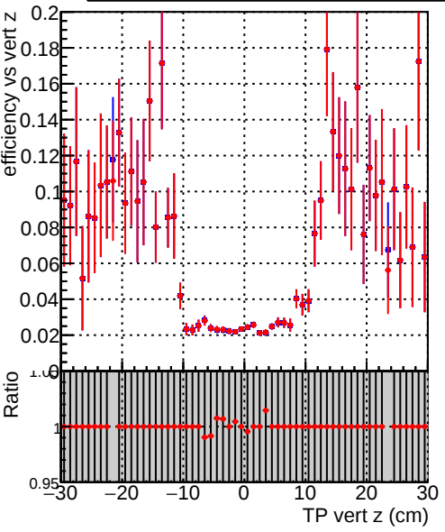
Efficiency vs TP vert z (cm) Legend: DQM_test_CKFFitDefault (blue line), DQM_test_doubleFit (red line)
