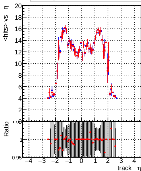
mean hits vs \eta Legend: DQM_test_CKFFitDefault (blue line), DQM_test_doubleFit (red line)
