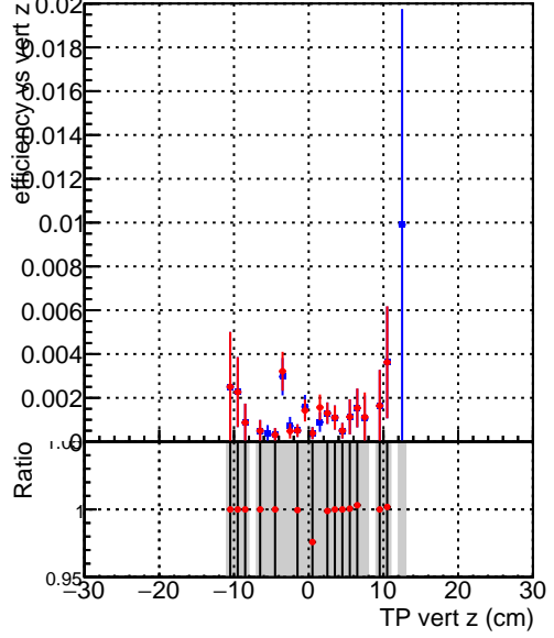
Efficiency vs vert z — DQM_test_CKFFitDefault (blue) — DQM_test_doubleFit (red)
