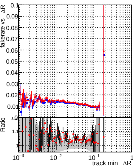
Fake rate vs \Delta R(\text{track}, \text{jet}) Legend: \blacksquare DQM_test_CKFFitDefault \bullet DQM_test_doubleFit
