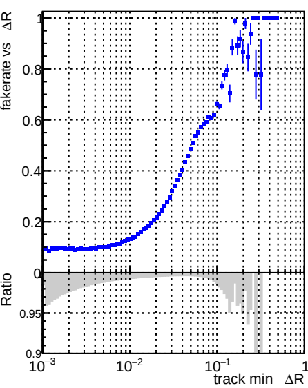
Fake rate vs \Delta R(\text{track, jet}) DQM_test_doubleFit
