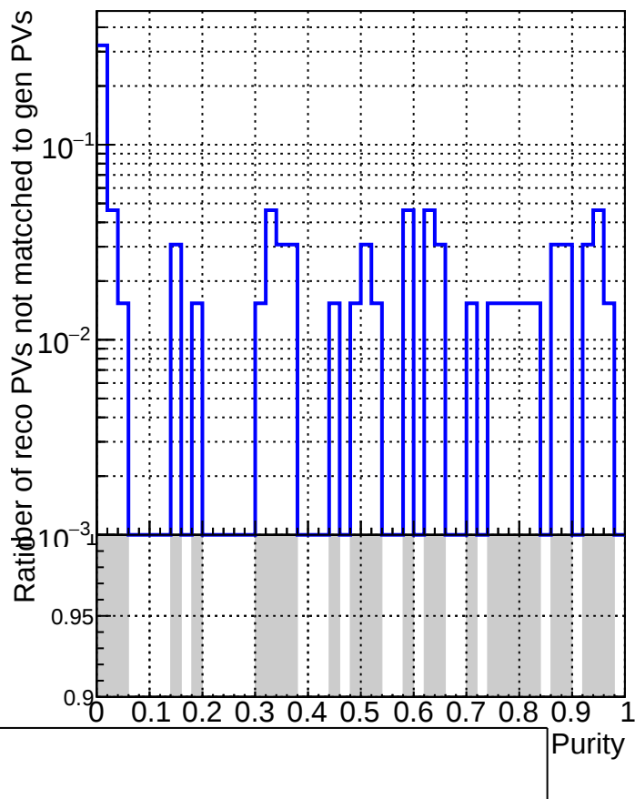
RecoPVAssoc2GenPVnotmatched_missing
