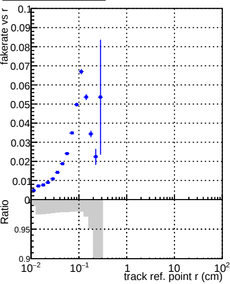
Fake rate vs vertpos DQM_test_doubleFit
