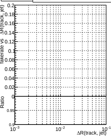
Fake rate vs \Delta R(\text{track, jet}) DQM_test_doubleFit
