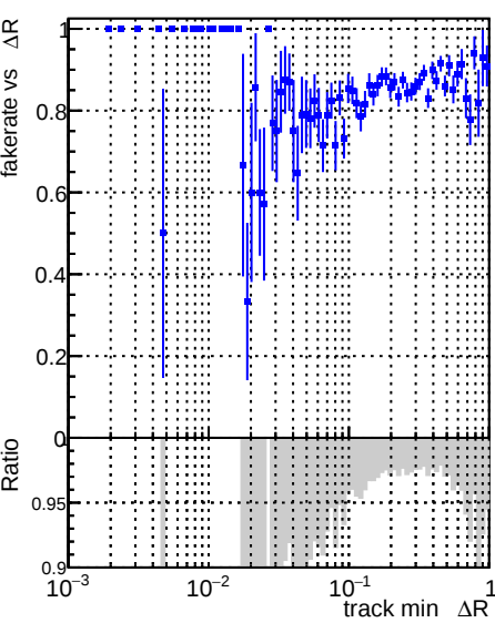
Fake rate vs \Delta R (track, jet) DQM_test_doubleFit
