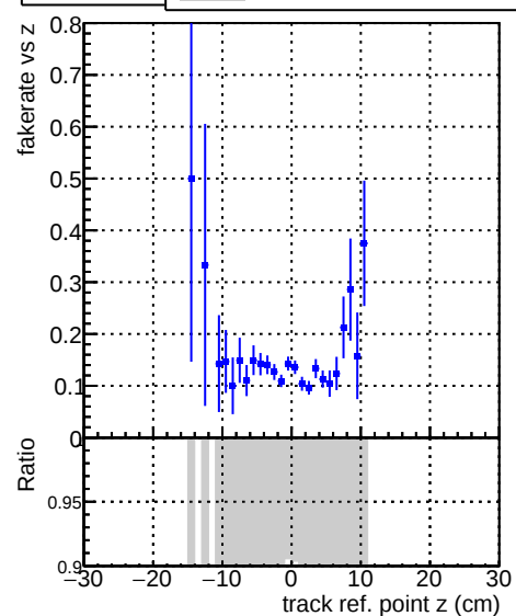
Fake rate vs v DQM_test_doubleFit
