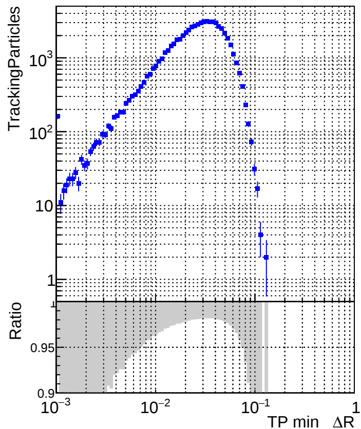
N of simulated tracks vs TP \Delta R(\text{TP, jet})
