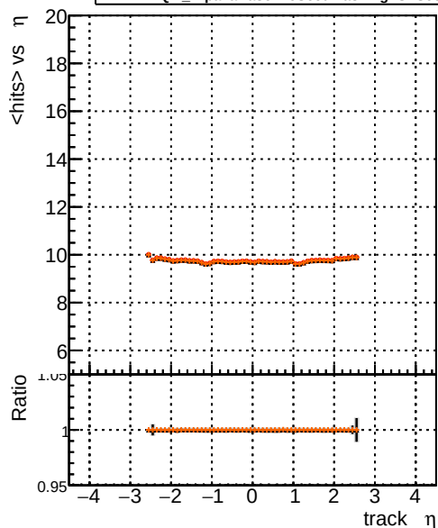
mean hits vs \eta — DQM_AlpaKaBaselineSeedMaskingLSTSeeding_HARVESTING — DQM_AlpaKaBaselineSeedMaskingLSTSeeding_mkFit_HARVESTING — DQM_AlpaKaBaselineSeedMaskingLSTSeeding_mkFitFIT_HARVESTING
