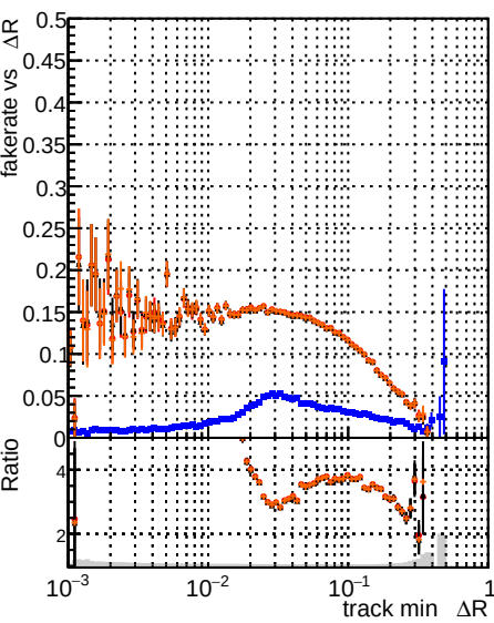
Fake rate vs \Delta R(\text{track, jet}) Legend: Iter1-legacyQuads-CKF Iter1-legacyTriplets-CKF Iter1-LS+Seed-CKFBuild-CKFFit Iter1-LS+Seed-MkFitBuild-MkFitFit Iter2-legacyQuads-CKF Iter2-legacyTriplets-CKF Iter2-LS+Seed-CKFBuild-CKFFit Iter2-LS+Seed-MkFitBuild-MkFitFit
