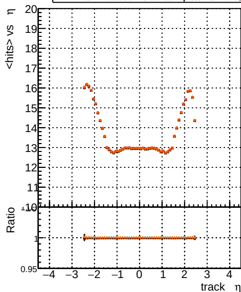
mean hits vs \eta — Iter1-Patatrack+CleanedTriplets-LSTBuild_Iter2-LSTSeed-CKFFit-Build-CKFFit — Iter1-Patatrack+CleanedTriplets-LSTBuild_Iter2-LSTSeed-MkFitBuild-CKFFit — Iter1-Patatrack+CleanedTriplets-LSTBuild_Iter2-LSTSeed-MkFitBuild-MkFitFit
